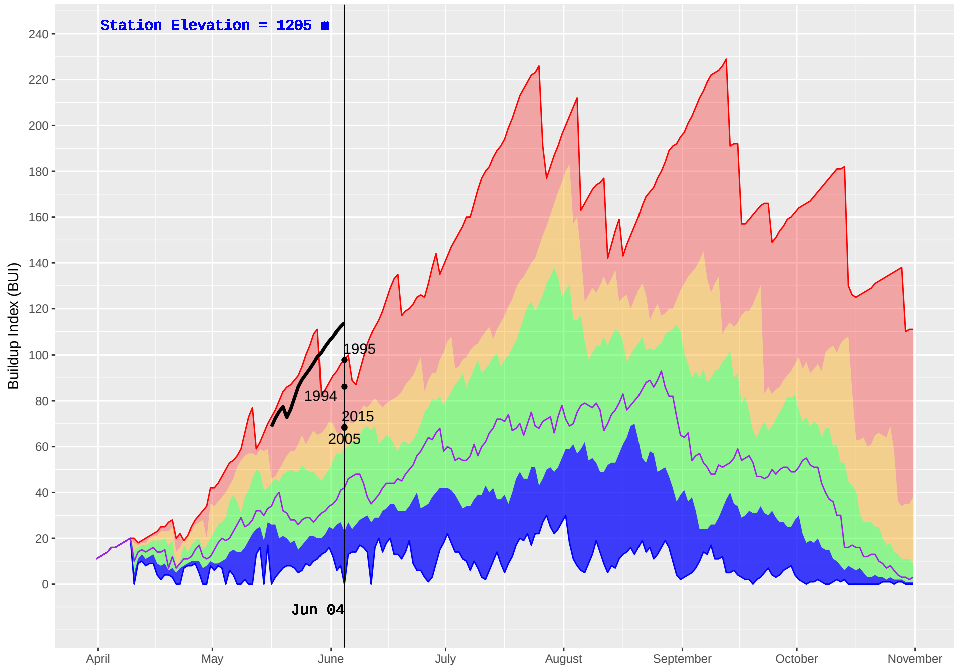
GWYNETH LAKE (309) : Historical (1986–2016) and Current (2018) Noon Buildup Index (BUI)
