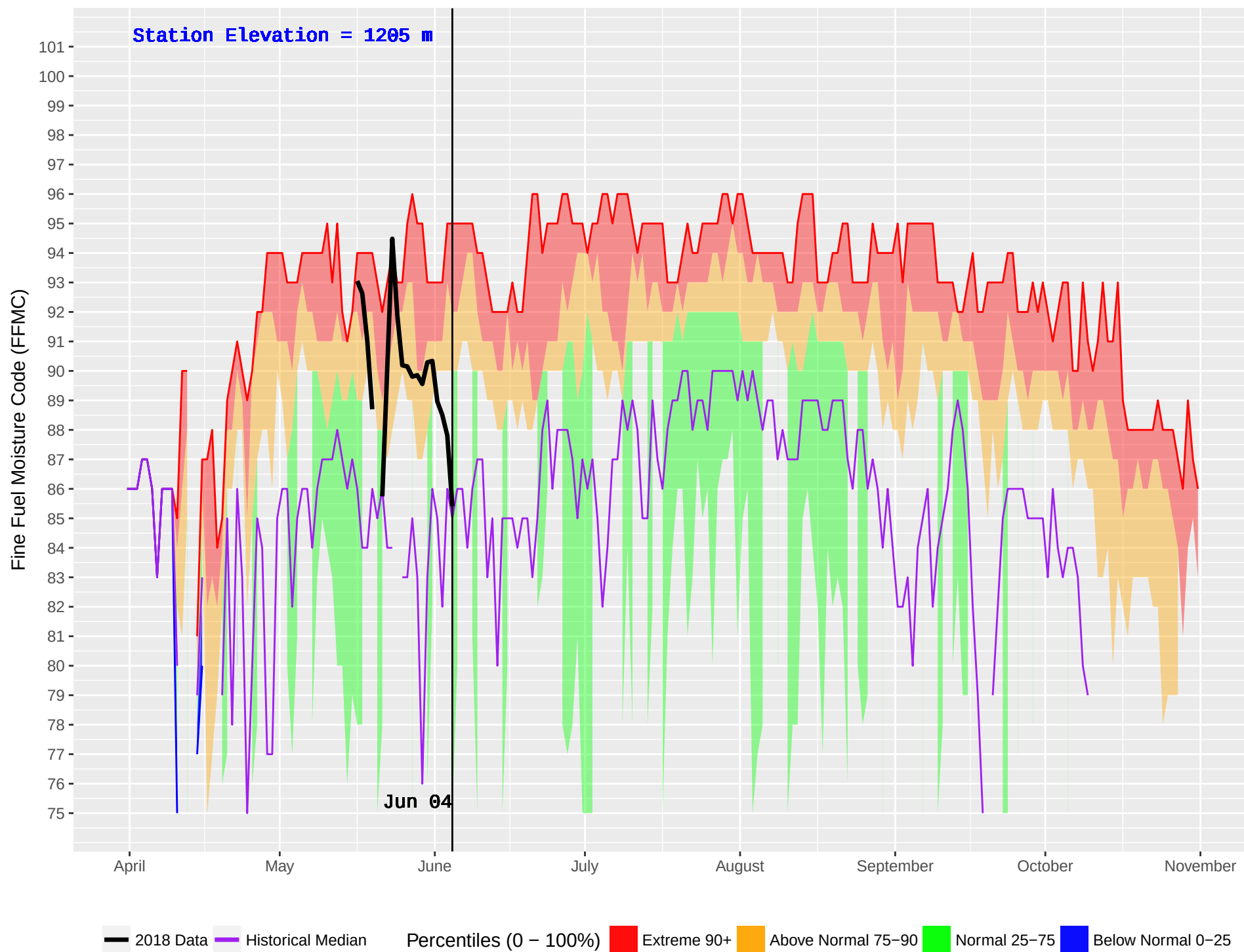
GWYNETH LAKE (309) : Historical (1986–2016) and Current (2018) Noon Fine Fuel Moisture Code (FFMC)
